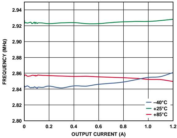
Figure 34. Buck Switching Frequency vs. Output Current, Across Temperature, V_{OUT1} = 1.8\text{ V} , PWM Mode
