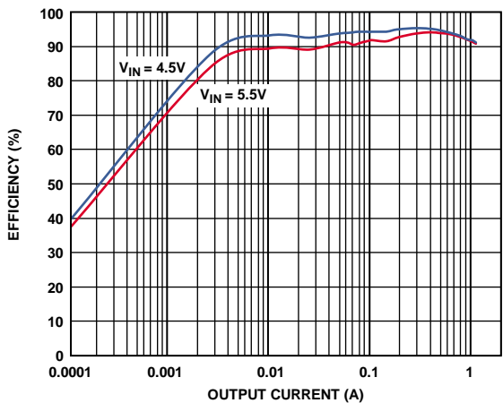
Figure 17. Buck Efficiency vs. Load Current, Across Input Voltage, V_{OUT1} = 3.8V , Auto Mode
