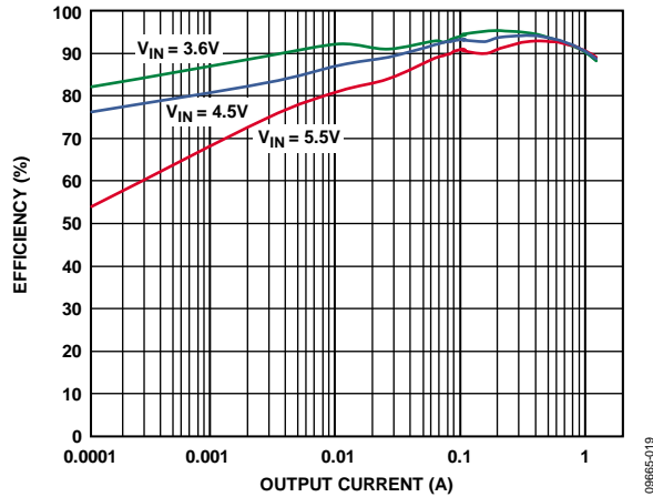
Figure 19. Buck Efficiency vs. Load Current, Across Input Voltage, V_{OUT1} = 3.3V , Auto Mode
