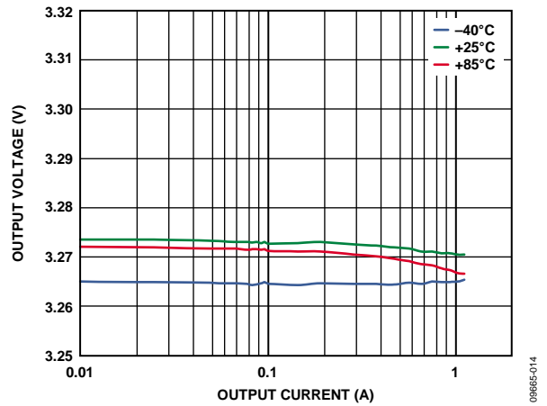
Figure 14. Buck Load Regulation Across Temperature, V_{OUT1} = 3.3 V , PWM Mode
