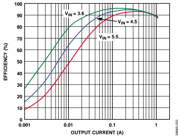
Figure 20. Buck Efficiency vs. Load Current, Across Input Voltage, V_{OUT1} = 3.3V , PWM Mode
