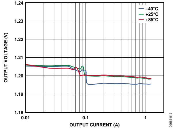
Figure 12. Buck Load Regulation Across Temperature, V_{OUT1} = 1.2 V , Auto Mode
