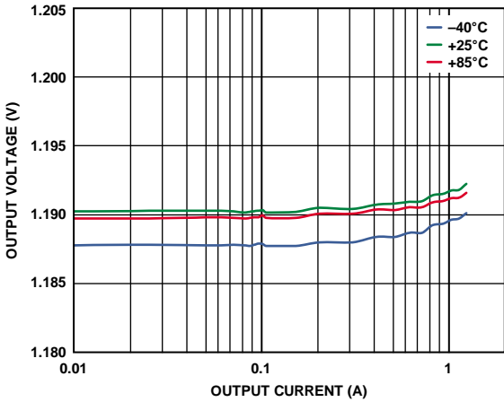
Figure 16. Buck Load Regulation Across Temperature, V_{OUT1} = 1.2V , PWM Mode
