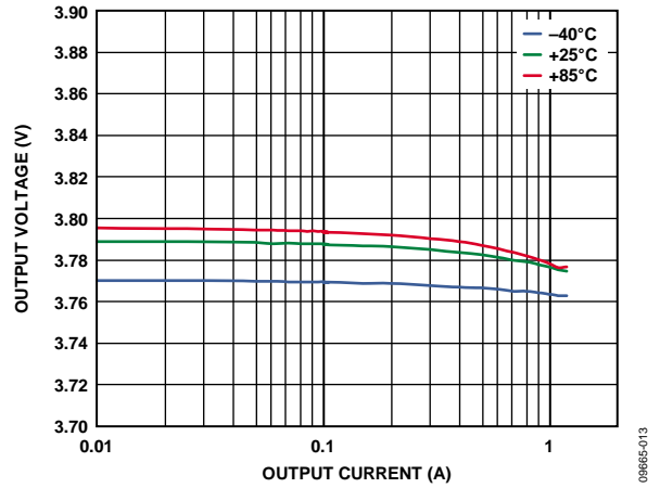
Figure 13. Buck Load Regulation Across Temperature, V_{OUT1} = 3.8 V , PWM Mode
