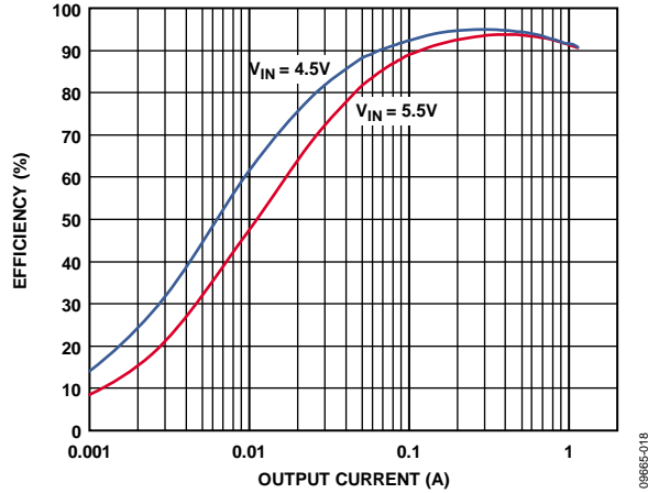
Figure 18. Buck Efficiency vs. Load Current, Across Input Voltage, V_{OUT1} = 3.8V , PWM Mode
