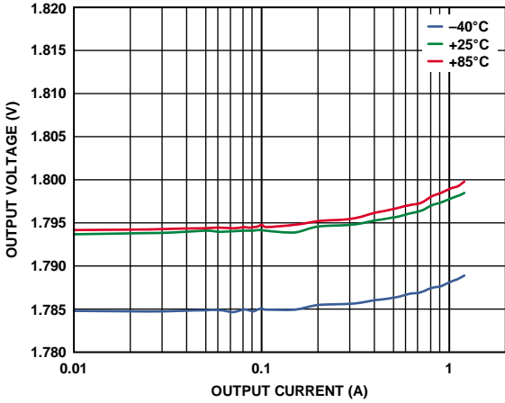
Figure 15. Buck Load Regulation Across Temperature, V_{OUT1} = 1.8V , PWM Mode
