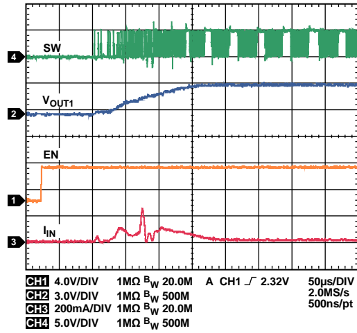
Figure 6. Buck Startup, VOUT1 = 3.3 V, IOUT2 = 20 mA
