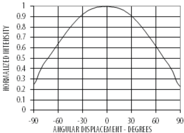
Figure 5 Radiation Pattern
