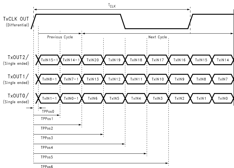
FIGURE 11. Transmitter LVDS Output Pulse Position Measurement
