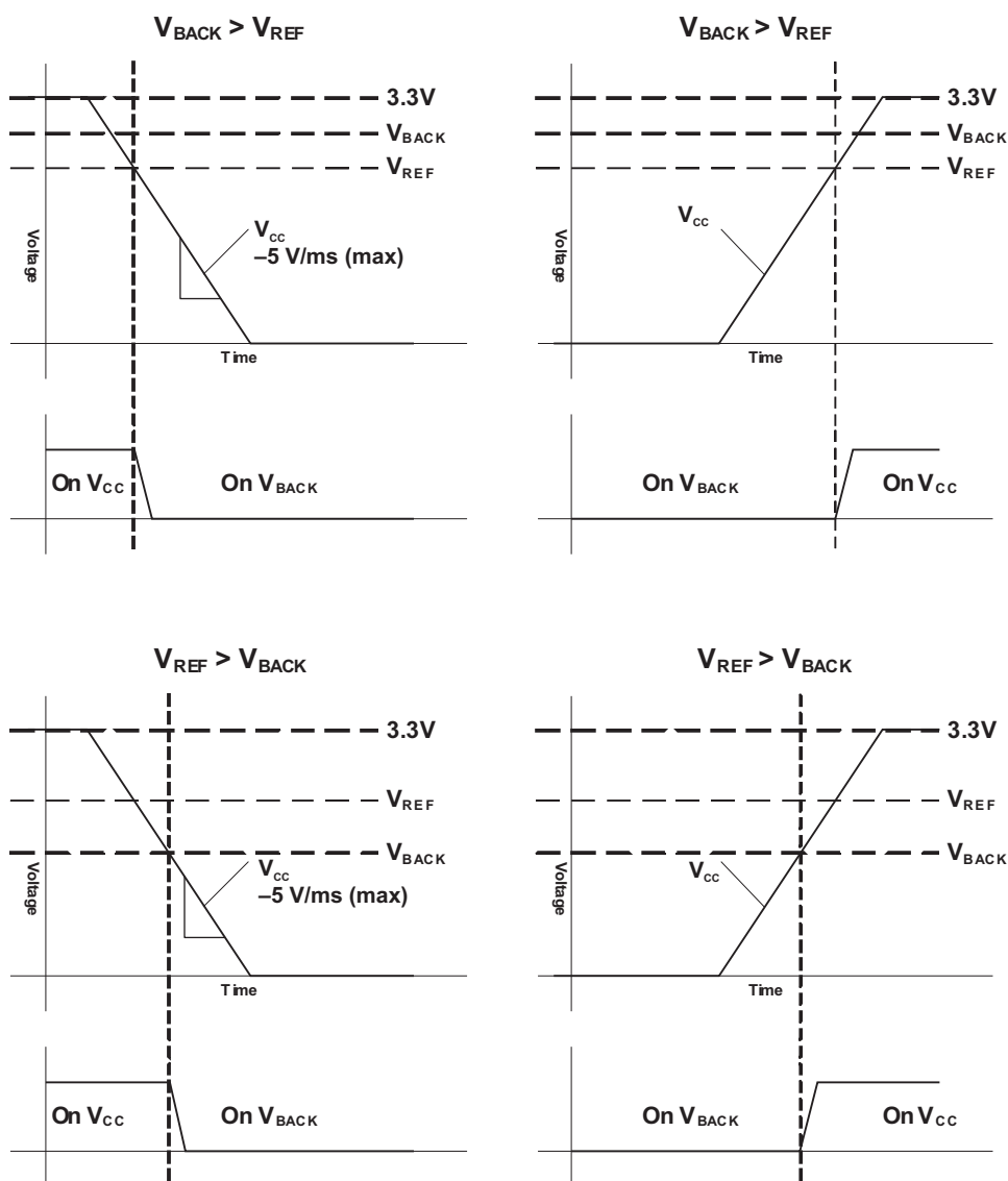
Figure 2. Switchover Diagram
