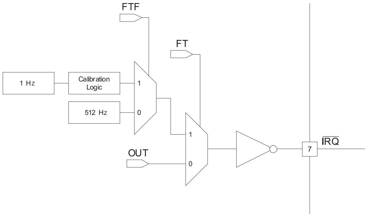
Figure 1. IRQ Pin Functional Diagram
