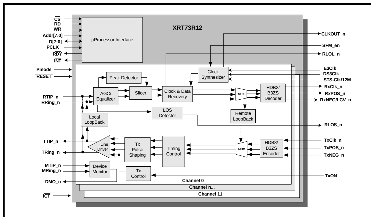
FIGURE 1. BLOCK DIAGRAM OF THE XRT 73R12
