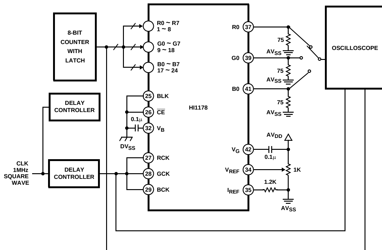
FIGURE 3. SETUP HOLD TIME AND GLITCH ENERGY TEST CIRCUIT
