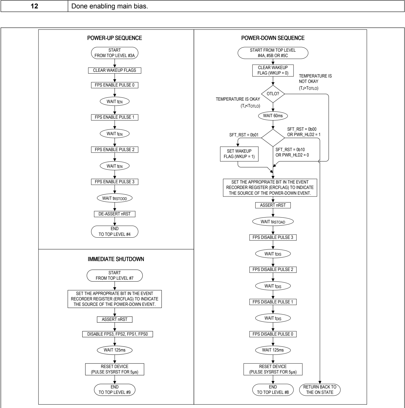
Figure 5. Power-Up/Down Sequence
