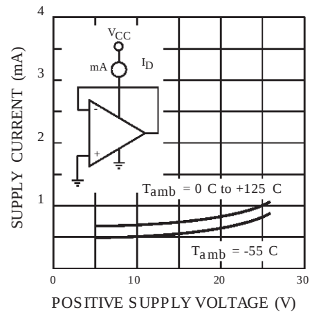
SUPPLY CURRENT
