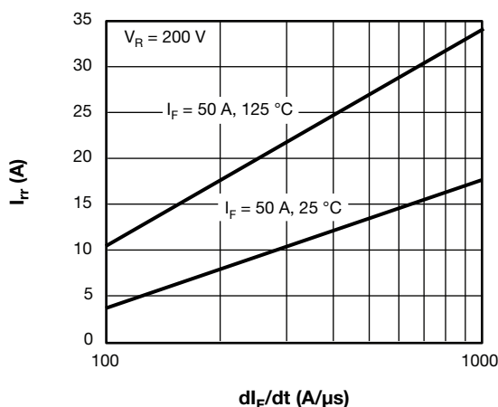
Fig. 9 - Typical I_{rr} Diode vs. dl_F/dt
