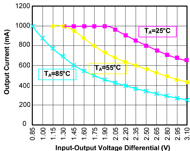
Figure 5-Safe Operation Area of EP1117 in SOT-223 and TO-252 packages (Limited by Power Dissipation with T_{JUNCTION} < 125^\circ\text{C} )
