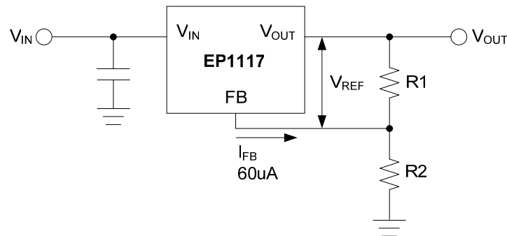
Figure 1-Basic Adjustable Regulator
