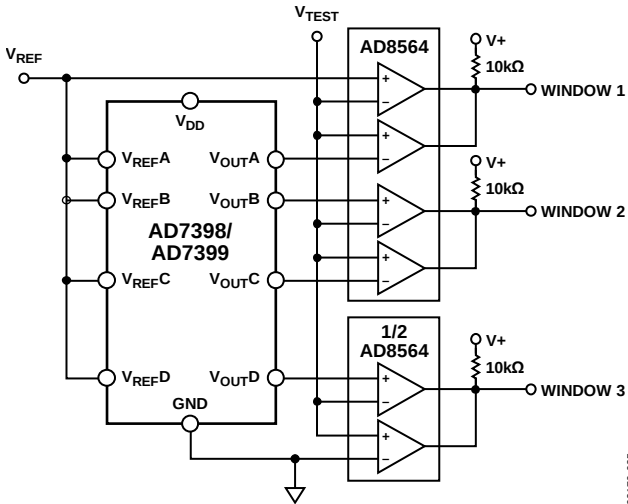
Figure 35. Overlapping Windows Comparator
