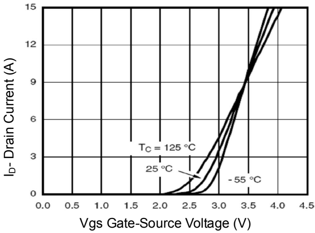
Figure 7 Transfer Characteristics
