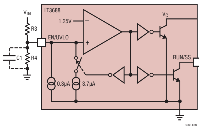
Figure 8. Undervoltage Lockout
