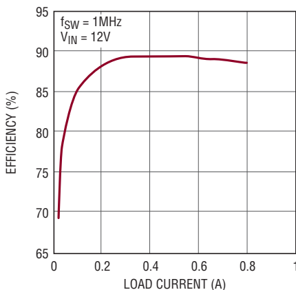
Efficiency, V_{\text{OUT}} = 5\text{V}
