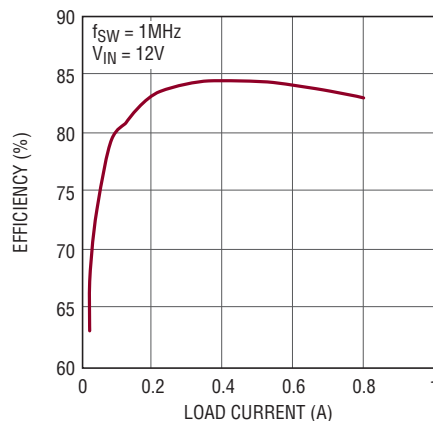
Efficiency, V_{\text{OUT}} = 3.3\text{V}
