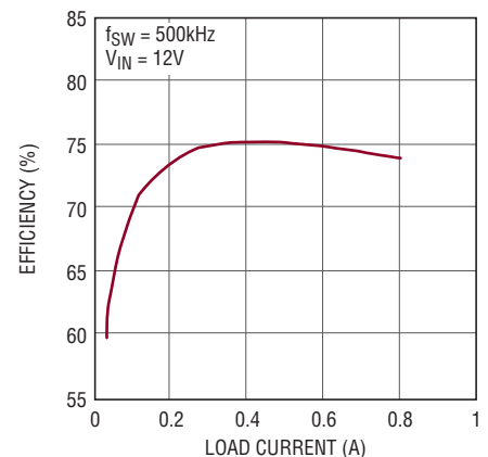
Efficiency, V_{\text{OUT}} = 1.8\text{V}
