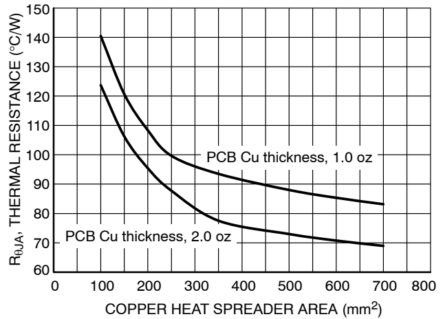
Figure 43. R θJA vs. PCB Copper Area (SOIC-8 EP)
