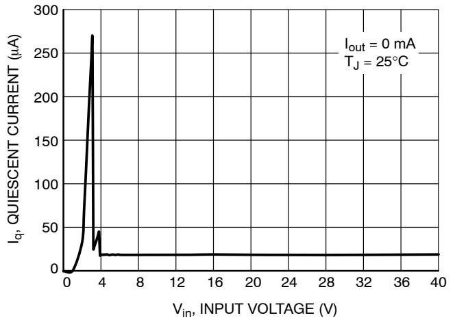
Figure 7. Quiescent Current vs. Input Voltage (3.3 V option)
