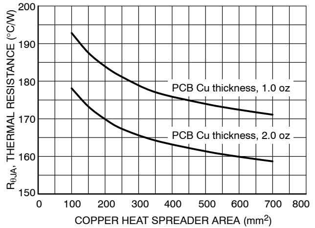
Figure 42. R θJA vs. PCB Copper Area (SOIC-8)
