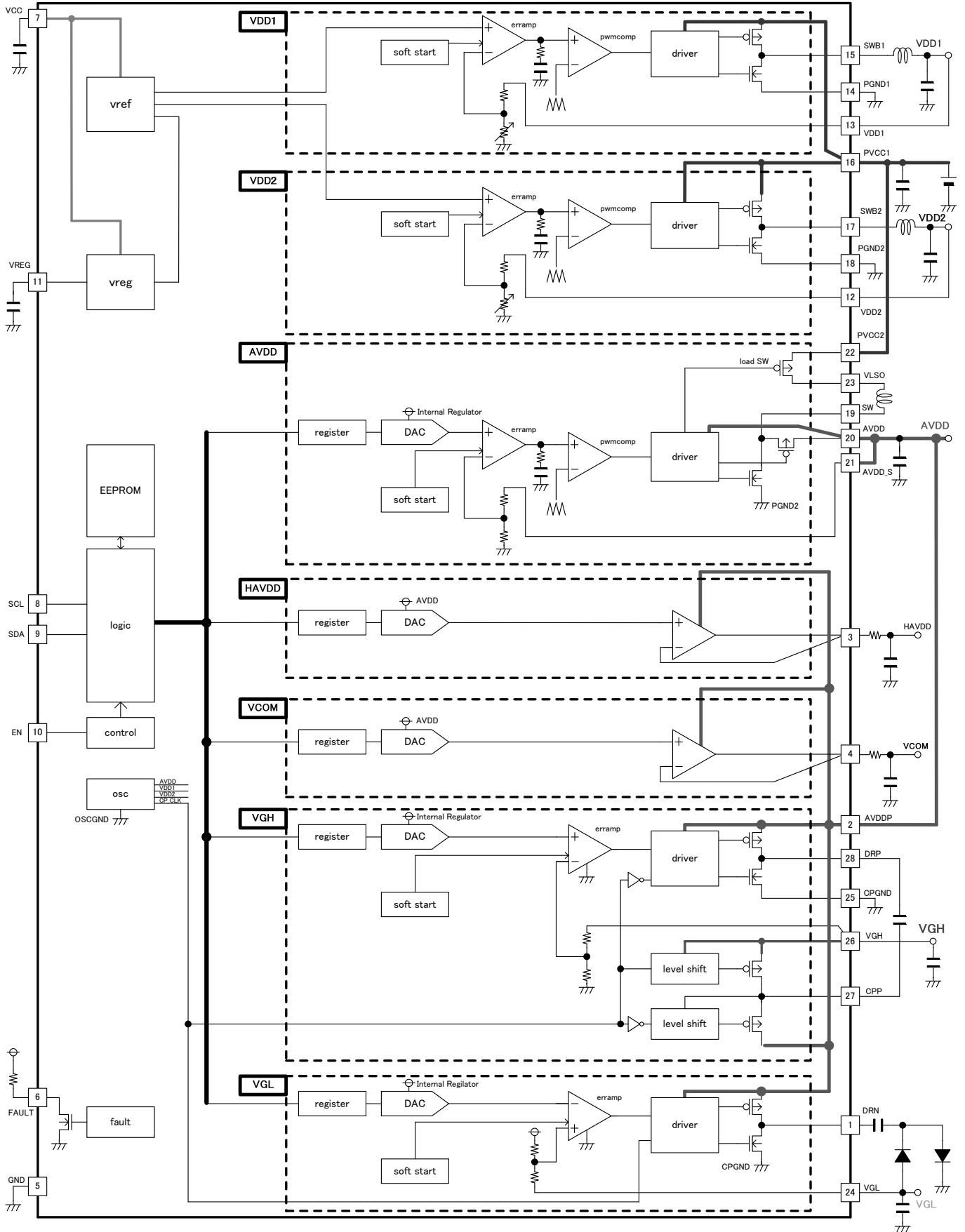
Fig.3 Block Diagram
