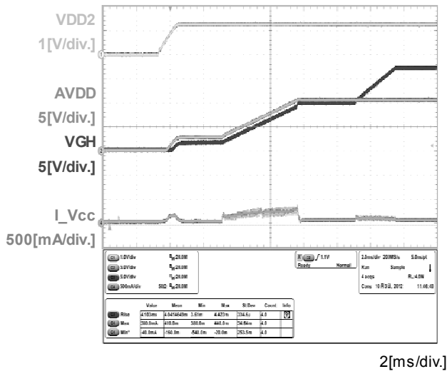
Fig.27 VGH Start-up Sequence
