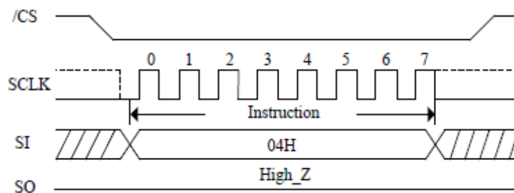
Figure 2. Write Disable Sequence Diagram
