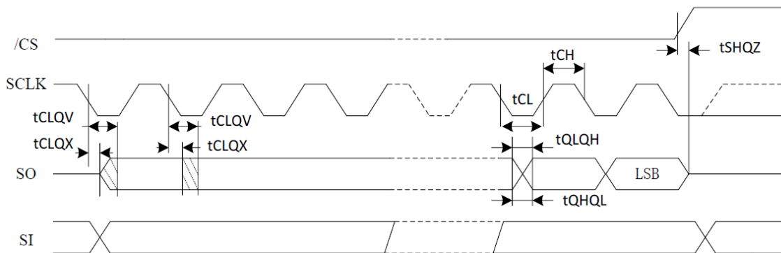
Figure 22. Output Timing
