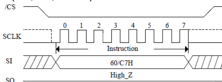
Figure 18. Chip Erase Sequence Diagram
