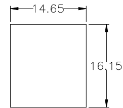
FRONT OPENNING
