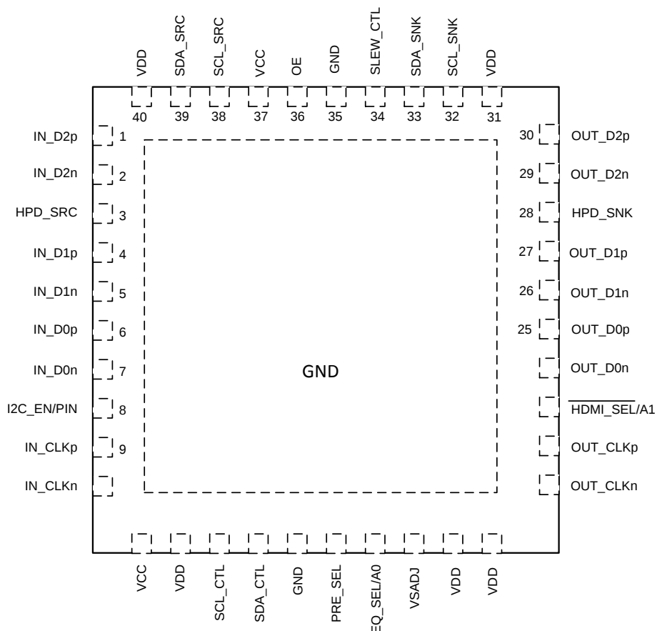
RSB Package 40-Pin WQFN Top View
