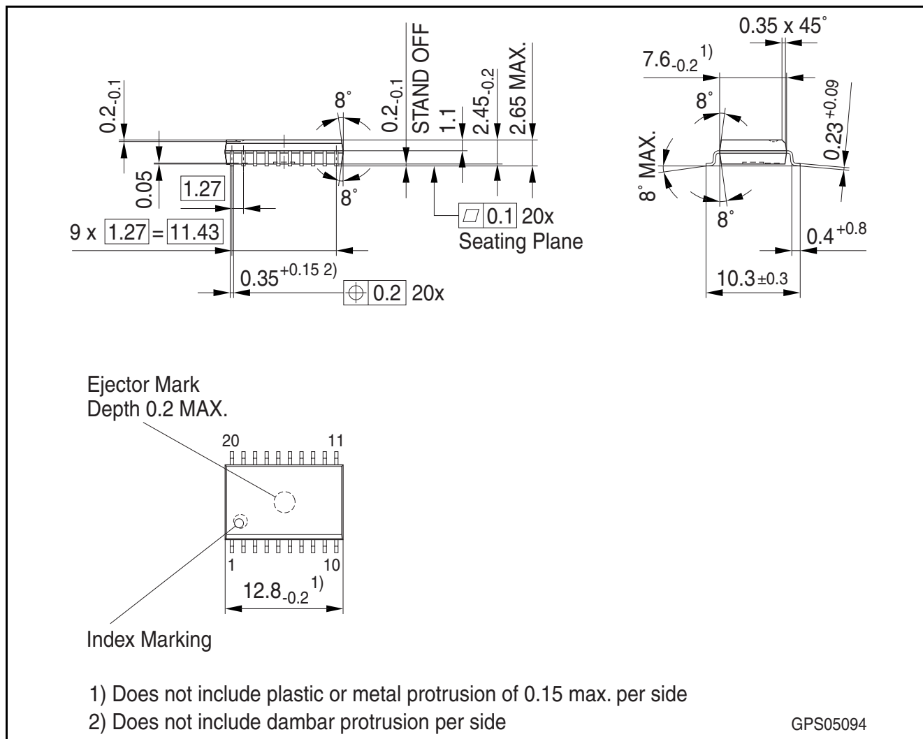
Figure 13 PG - DSO20-45 (Plastic Green Dual Small Outline Package)
