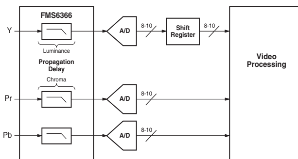
Figure 2: Digital Delay Compensation for anti-alias 4:2:2 filters
