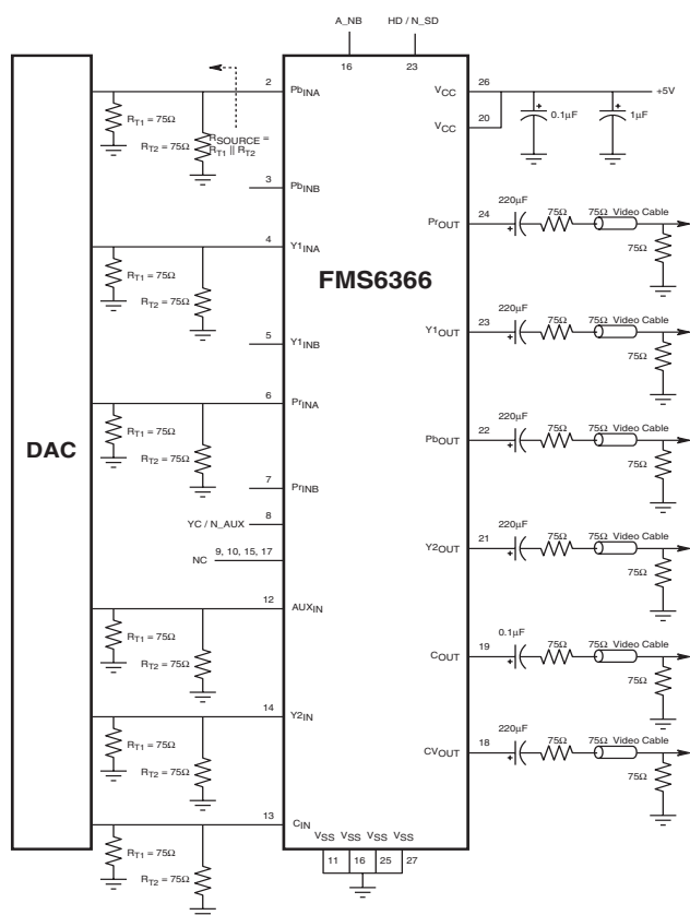
Figure 1: Typical Application Diagram
