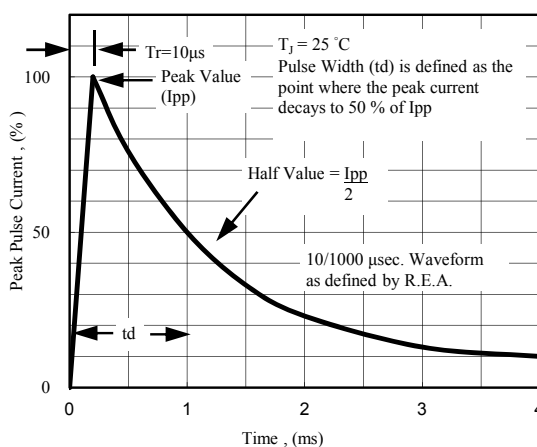
Fig. 5 - Pulse Waveform
