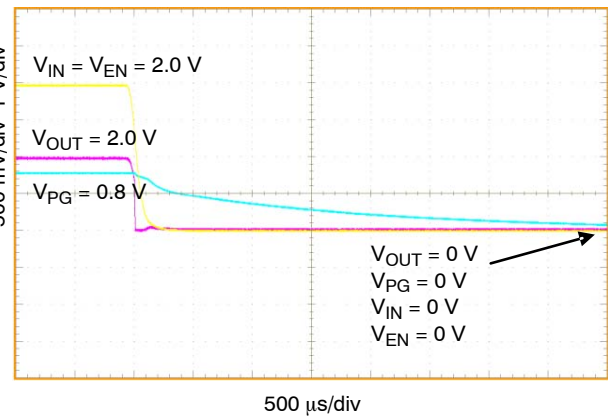
Figure 46. Input Voltage Turn-off Response NCP752B, V_{OUT} = 0.8 \text{ V}
