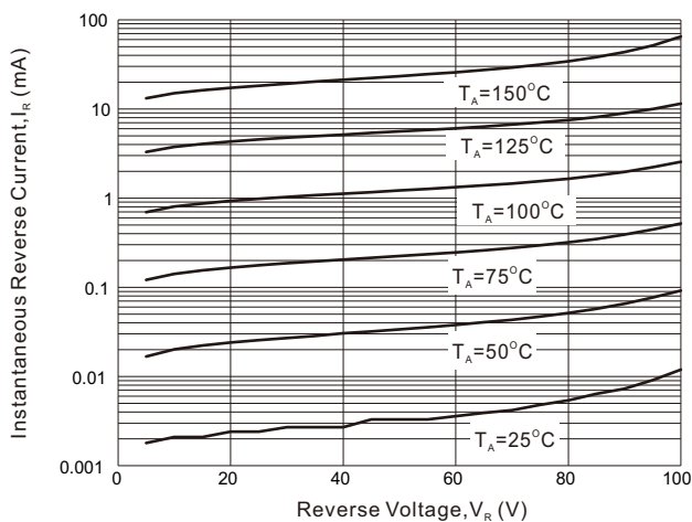
Fig. 2 - Reverse Characteristics (per diode)
