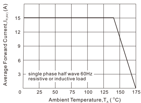
Fig.3 - Forward Current Derating Curve (per diode)
