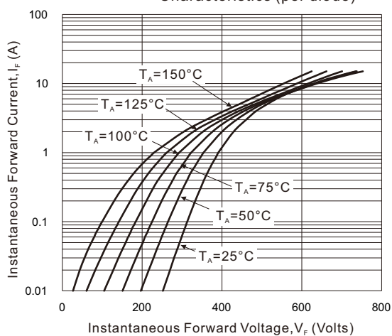
Fig. 1 - Instantaneous Forward Characteristics (per diode)
