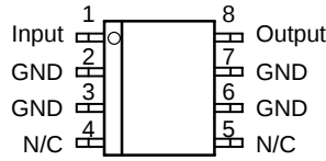
MC33275D
