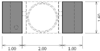
Reverse Mount
