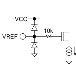
Figure 45. VREF
