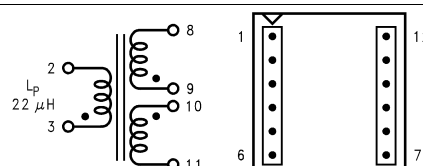
Figure 34. T4 - Top View Coilcraft Q4344-B
