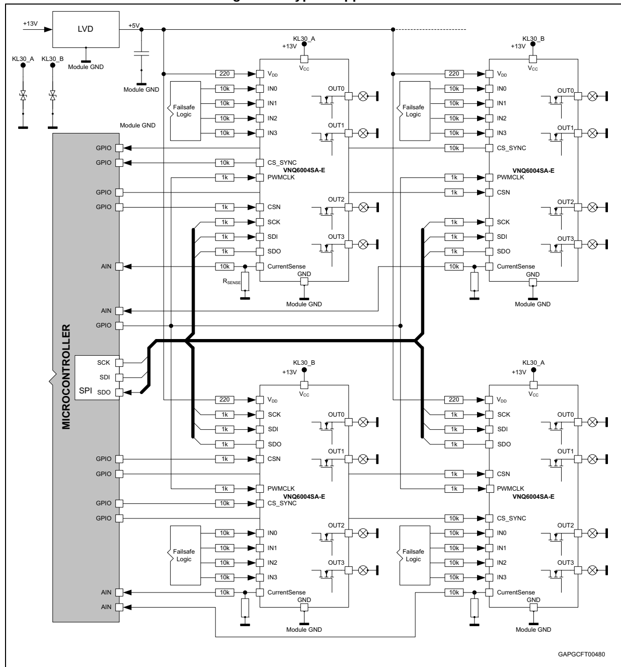
Figure 24. Typical application
