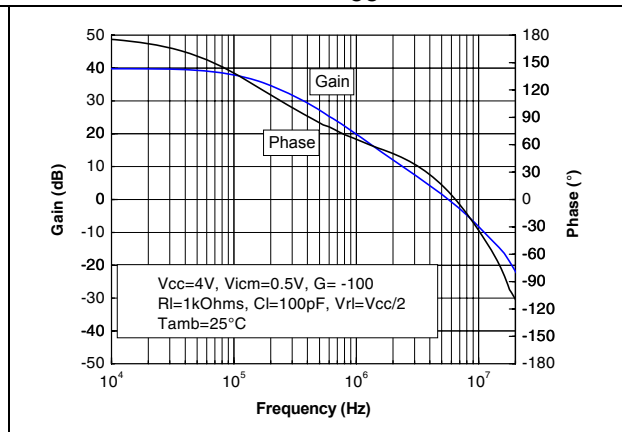
Figure 16. Voltage gain and phase vs. frequency at V_{CC}=4\text{ V} , V_{icm}=0.5\text{ V}
