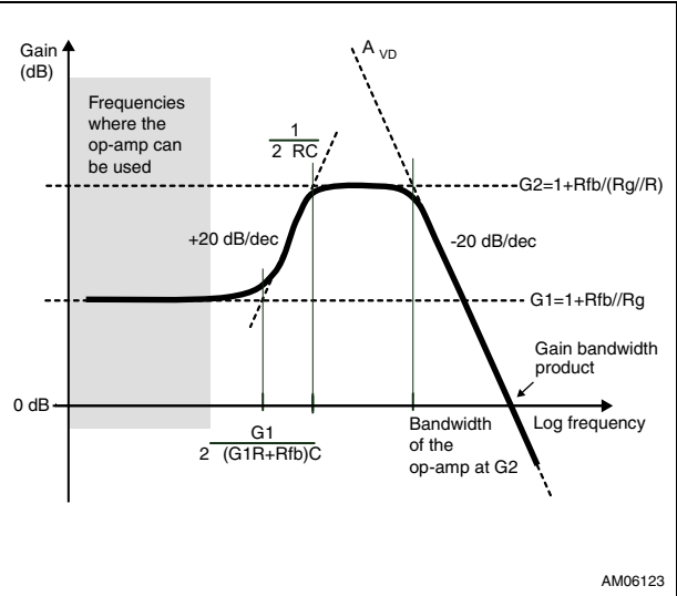
Figure 25. Closed-loop gain
