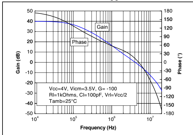
Figure 15. Voltage gain and phase vs. frequency at V_{CC}=4\text{ V} , V_{icm}=3.5\text{ V}
