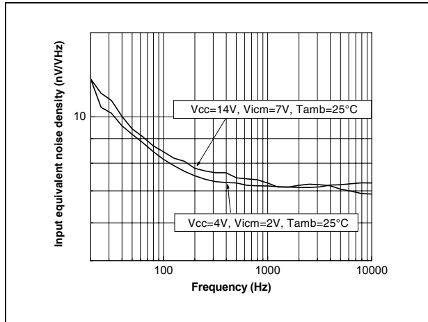
Figure 13. Noise vs. frequency at V_{CC}=4\text{ V} and V_{CC}=14\text{ V}
