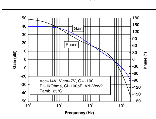
Figure 17. Voltage gain and phase vs. frequency at V_{CC}=14\text{ V} , V_{icm}=7\text{ V}
