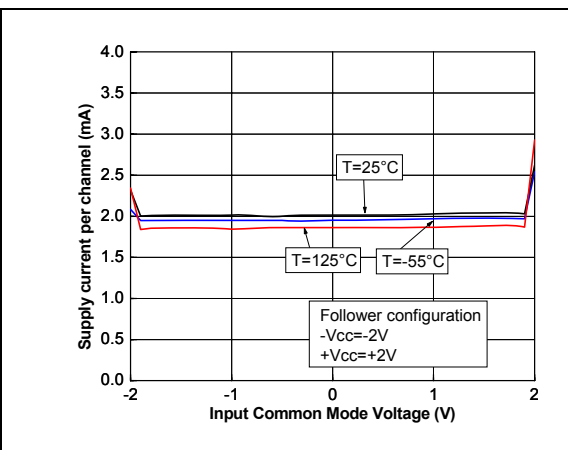
Figure 5. Supply current vs. Vicm in follower configuration at V CC = 4 V
