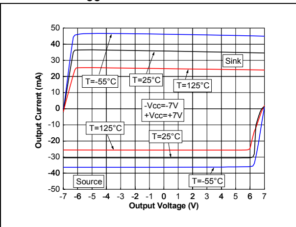
Figure 10. Output current vs. output voltage at V_{CC} = 14\text{ V}
