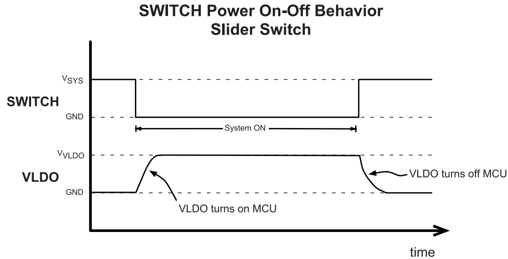
图 2-15. SWITCH, Slider Power On-Off Behavior
