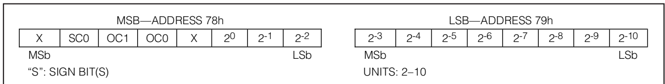
Figure 9. RSGAIN Register
