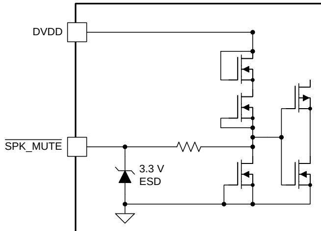
Figure 13. SPK_MUTE Pin
