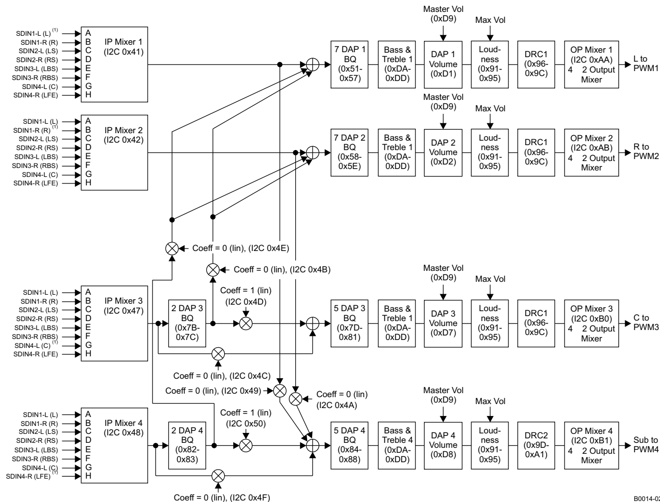
Figure 1-2. TAS5504A DAP Architecture With I 2 C Registers ( f_s \leq 96 kHz)
