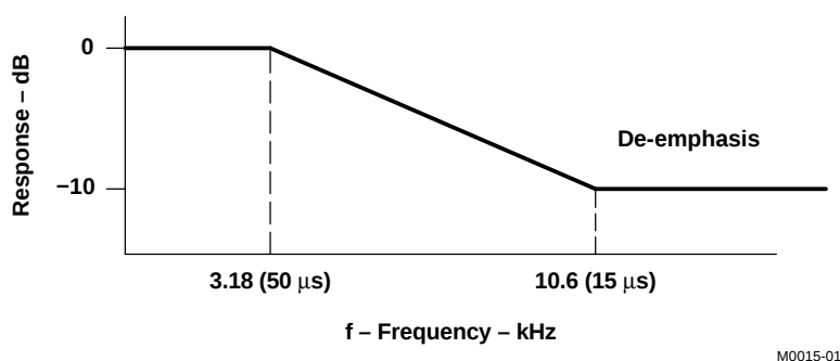
Figure 1-21. De-Emphasis Filter Characteristics
