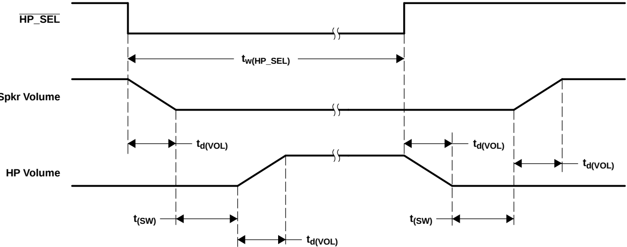
Figure 3-9. \overline{\text{HP\_SEL}} Timing
