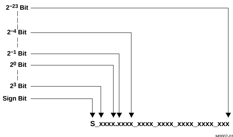
Figure 1-5. 5.23 Format
