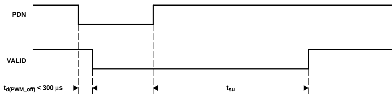
Figure 3-6. Power-Down Timing
