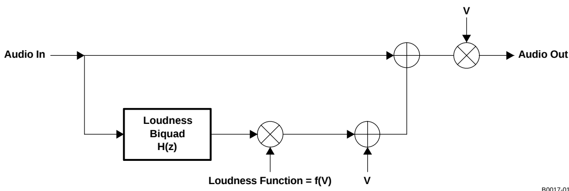
Figure 1-15. Loudness Compensation Functional Block Diagram
