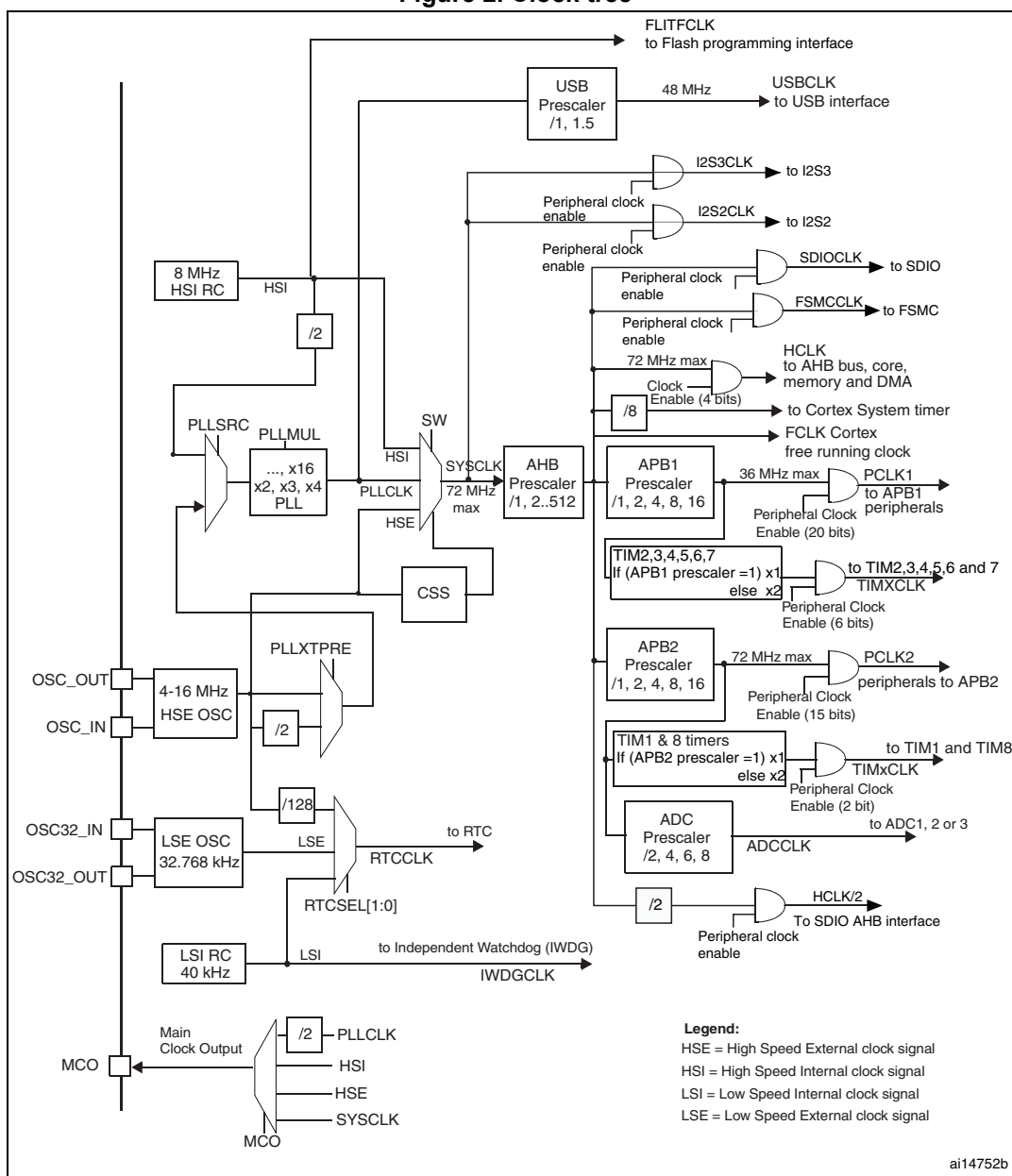
Figure 2. Clock tree
