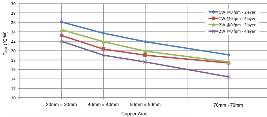
Figure 9-2. Measured R_{\theta JA} versus PCB Copper Area on 2-Layer Boards and 4-Layer Boards
