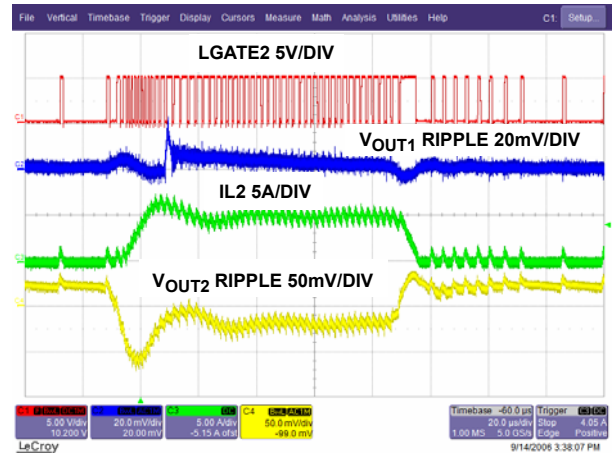
FIGURE 47. LOAD TRANSIENT V_{OUT1} = 3.3V (SKIP)
