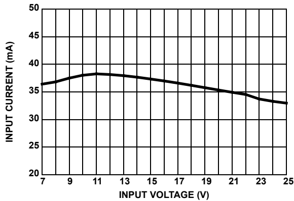
FIGURE 31. PWM NO LOAD INPUT CURRENT vs V_{IN} ( EN = EN2 = EN\_LDO = VCC )
