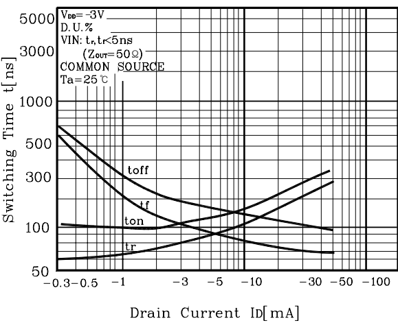
Fig8 t - Id
