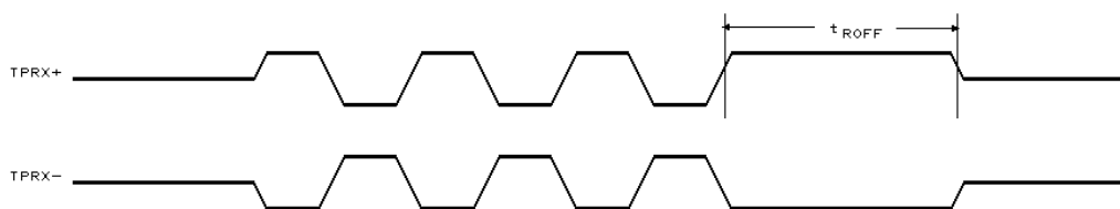
Receive Timing
