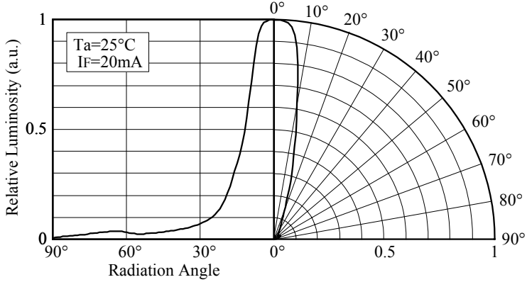
■ Directivity (NSPW300BS)
