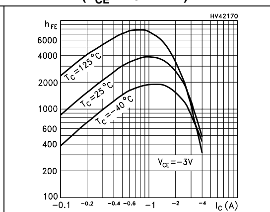
Figure 3. DC current gain ( V_{\text{CE}} = -3\text{ V PNP} )
