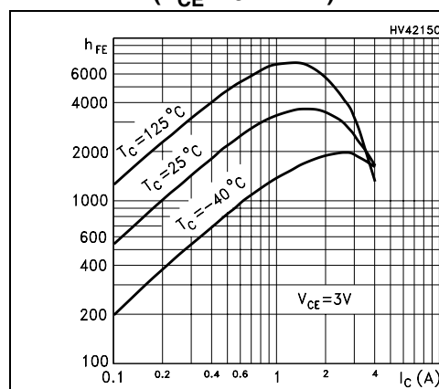
Figure 2. DC current gain ( V_{\text{CE}} = 3\text{ V NPN} )
