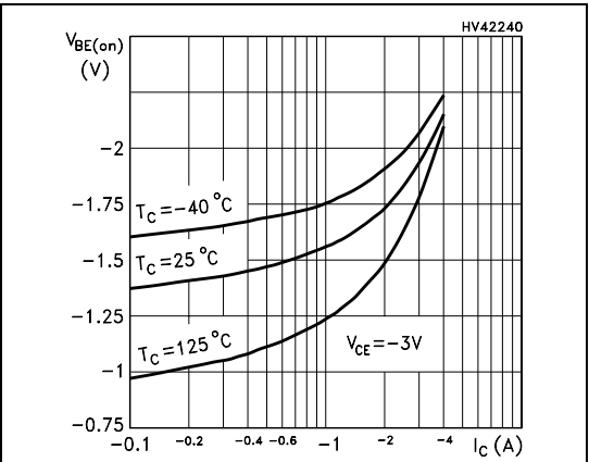
Figure 11. Base-emitter on voltage (PNP)
