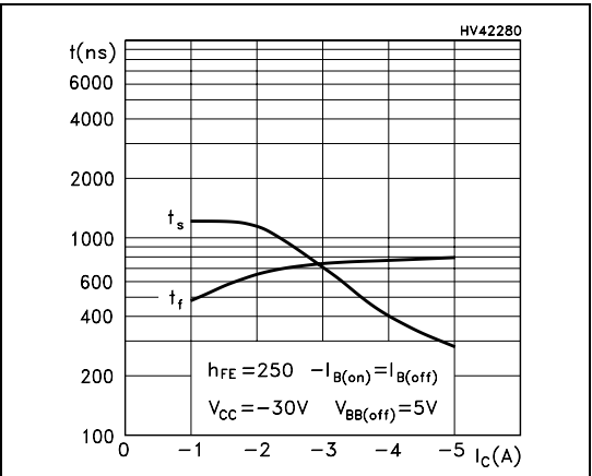
Figure 15. Resistive load switching time (PNP, off)
