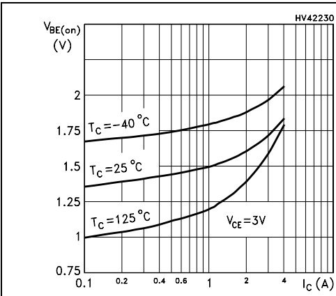
Figure 10. Base-emitter on voltage (NPN)
