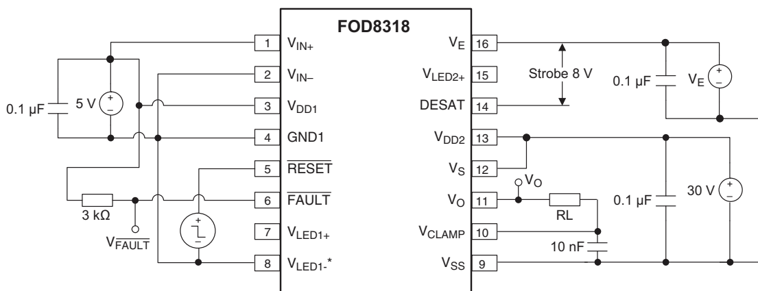
Figure 45. Reset Delay ( t_{\text{RESET}(\overline{\text{FAULT}})} ) Test Circuit
