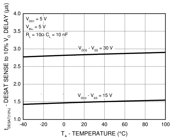
Figure 24. DESAT Sense to 10% V_O Delay ( t_{DESAT(10\%)} ) vs. Temperature
