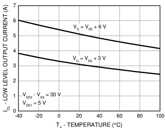
Figure 3. Low Level Output Current ( I_{\text{OL}} ) vs. Temperature
