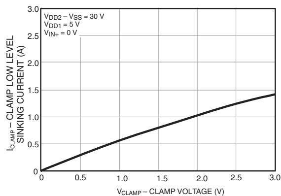
Figure 34. Clamp Low Level Sinking Current ( I_{CLAMP} ) vs. Clamp Voltage ( V_{CLAMP} )
