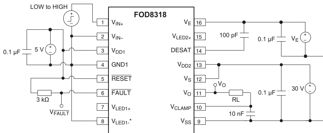
Figure 44. DESAT Sense ( t_{\text{DESAT}(90\%)} , t_{\text{DESAT}(10\%)} ), DESAT Fault ( t_{\text{DESAT}(\overline{\text{FAULT}})} ), and ( t_{\text{DESAT}(\text{LOW})} ) Test Circuit
