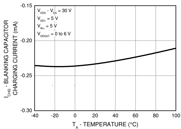
Figure 12. Blanking Capacitor Charge Current ( I_{CHG} ) vs. Temperature
