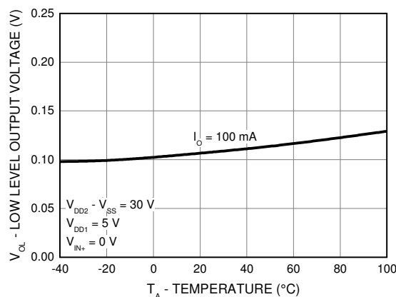
Figure 6. Low Level Output Voltage ( V_{\text{OL}} ) vs. Temperature
