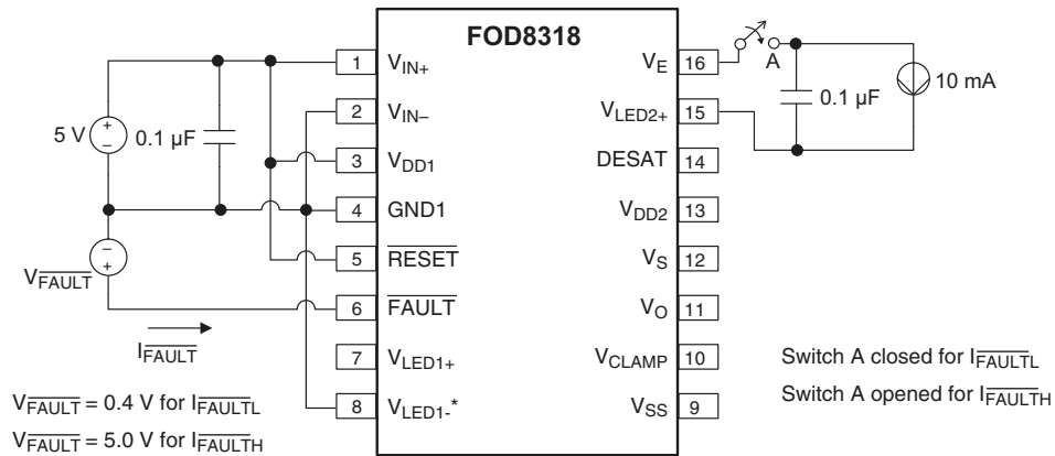
Figure 35. Fault Output Current ( I_{FAULTL} ) and ( I_{FAULTH} ) Test Circuit
