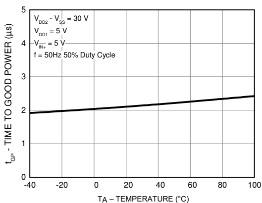
Figure 31. Time to Good Power ( t_{GP} ) vs. Temperature
