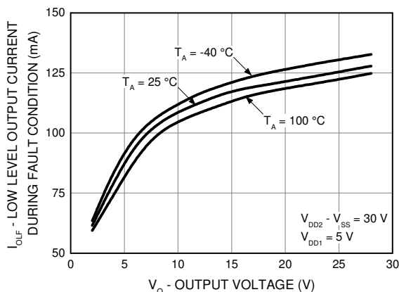
Figure 4. Low Level Output Current During Fault Condition ( I_{\text{OLF}} ) vs. Output Voltage ( V_{\text{OL}} )
