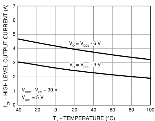
Figure 2. High Level Output Current ( I_{\text{OH}} ) vs. Temperature
