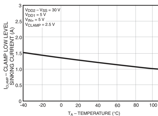
Figure 32. Clamp Low Level Sinking Current ( I_{CLAMP} ) vs. Temperature
