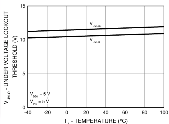
Figure 15. Under Voltage Lockout Threshold ( V_{UVLO} ) vs. Temperature
