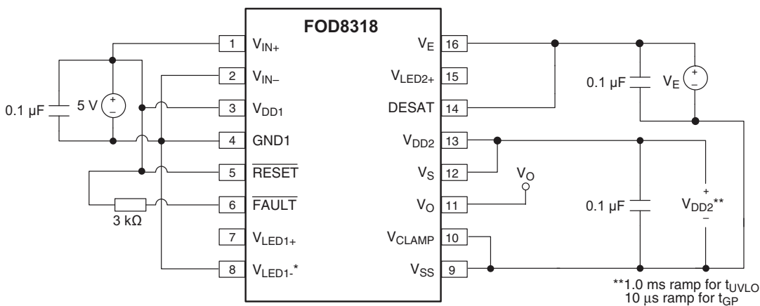
Figure 46. Under-Voltage Lockout Delay ( t_{\text{UVLO}} ) and Time to Good Power ( t_{\text{GP}} ) Test Circuit
