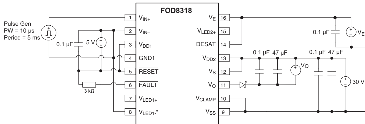
Figure 35. Fault Output Current ( I_{FAULTL} ) and ( I_{FAULTH} ) Test Circuit
