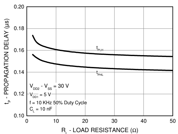
Figure 22. Propagation Delay ( t_P ) vs. Load Resistance ( R_L )
