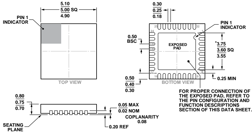
Figure 59. 32-Lead Lead Frame Chip Scale Package [LFCSP_WQ] 5 mm x 5 mm Body, Very Thin Quad (CP-32-12) Dimensions shown in millimeters
