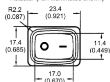
Actuator (non-illuminated shown)
