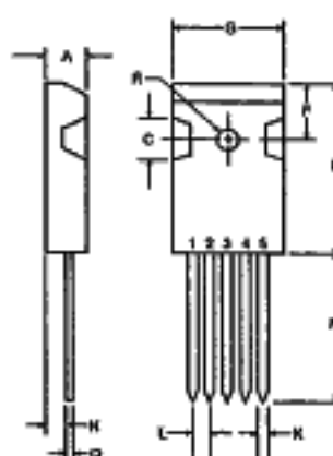
TO-247 (5 LEADED)
