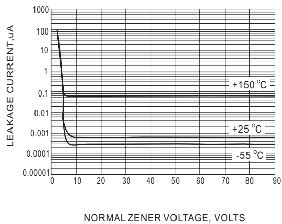
Fig.3 TYPICAL LEAKAGE CURRENT
