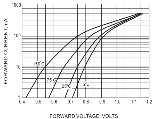
Fig.4 TYPICAL FORWARD VOLTAGE
