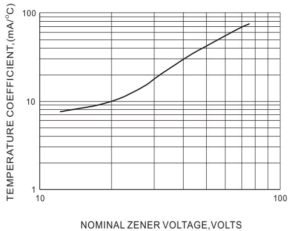
Fig.2 TEMPERATURE COEFFICIENTS
