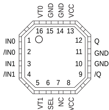
16-Pin MLF™
