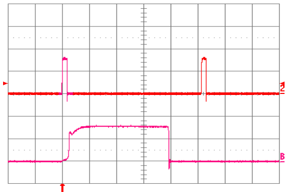
Figure 25. Load current (top trace, 20 A/div, 20 ms/div) into a 10 m \Omega short circuit during restart, at V_{in} = 48 V. Bottom trace (20 A/div, 1 ms/div) is an expansion of the on-time portion of the top trace.
