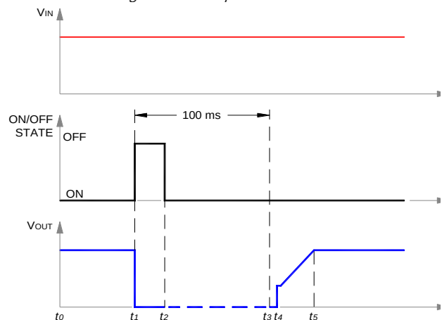
Figure 8. Startup scenario #3.
