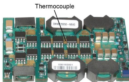
Figure 5. Location of the thermocouple for thermal testing
