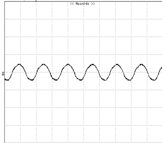
Figure 11: Input Terminal Ripple Current, i_c , at full rated output current and nominal input voltage with 12\mu\text{H} source impedance and 33\mu\text{F} electrolytic capacitor (500 mA/div, 2 us/div)
