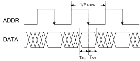
Address Shift-in Cycle
