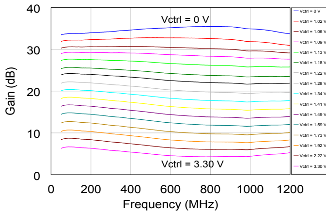
Gain Flatness Deviation ( 50 ~ 1000 MHz )
