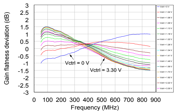
Gain Flatness Deviation ( 50 ~ 860 MHz )
