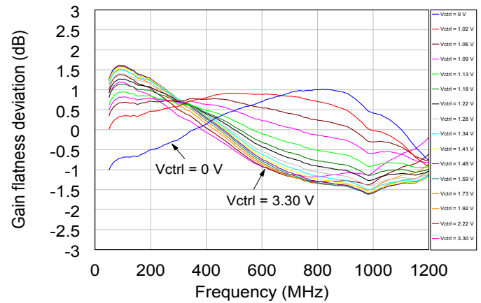
Gain Flatness Deviation ( 50 ~ 1200 MHz )
